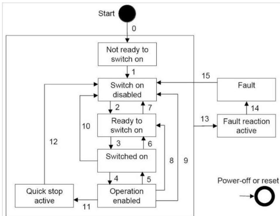
Figure 5-3. Power Drive System State Diagram
