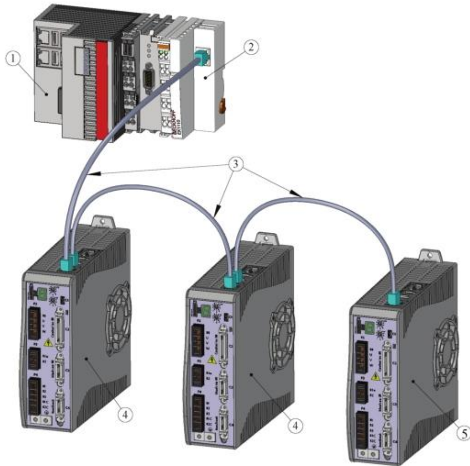
Figure 2-5. CDHDE-EtherCAT Configuration-Beckhoff Controller Example
