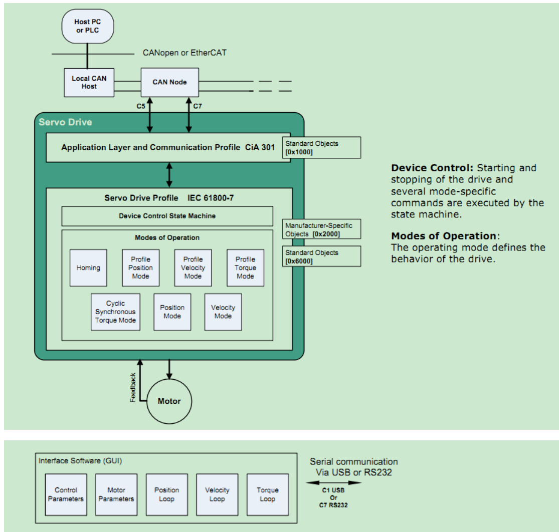
Figure 5-1. Communication Architecture
